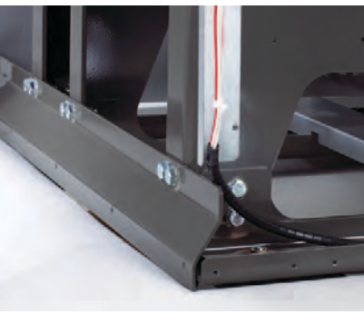
M-Series hard-mount washer design
